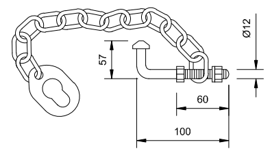
CHAIN LENGTH = 380 (12 LINKS + 1 RING) GATE CATCH N.T.S
