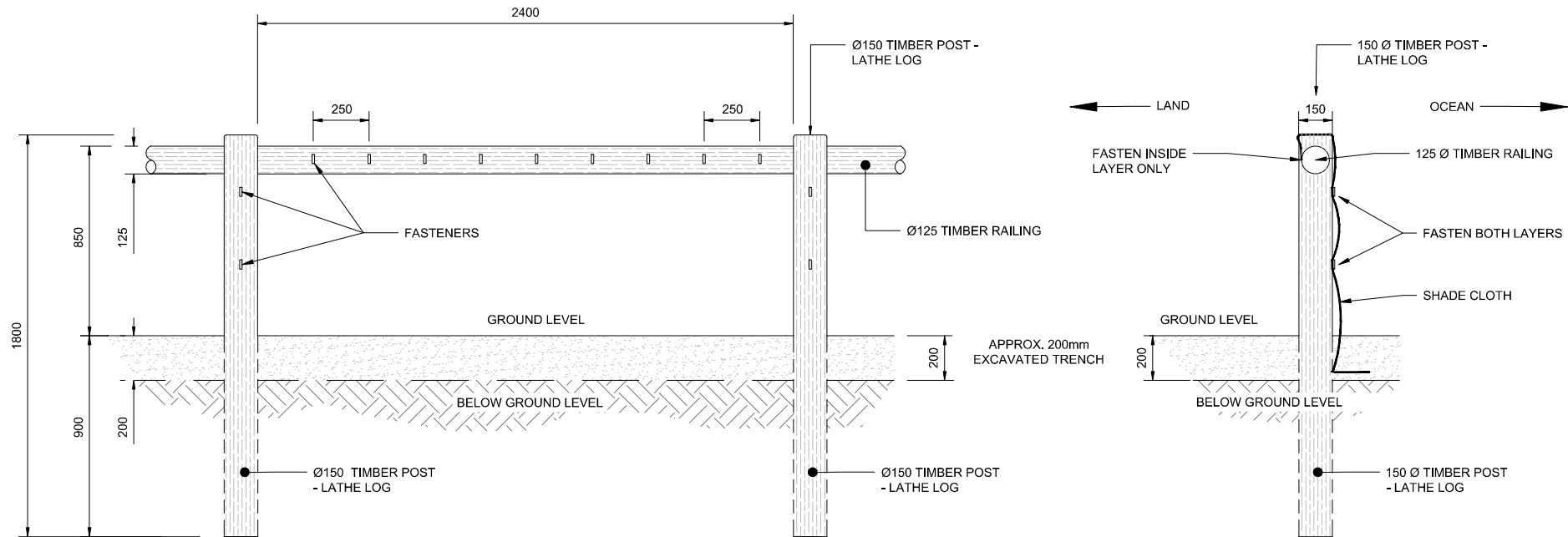
SIDE VIEW SCALE 1:20
