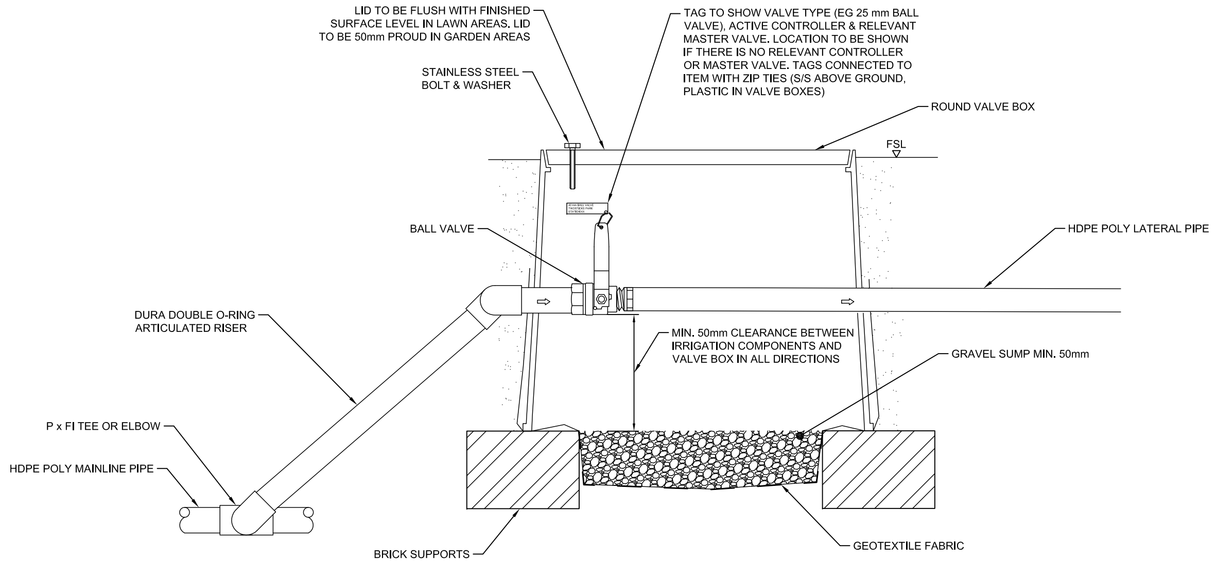
TYPICAL ISOLATION VALVE INSTALLATION (FOR MANUAL LATERAL ISOLATION)
