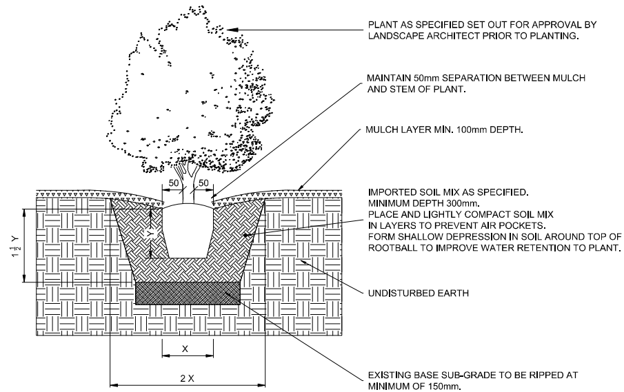
<300mm POT SIZE PLANT - PLANTING DETAIL NOT TO SCALE
