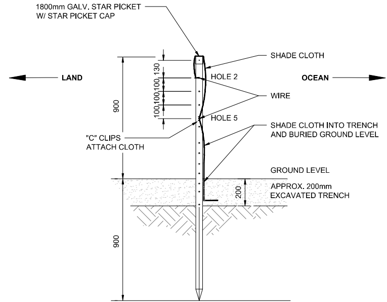
SIDE VIEW SCALE 1:20
