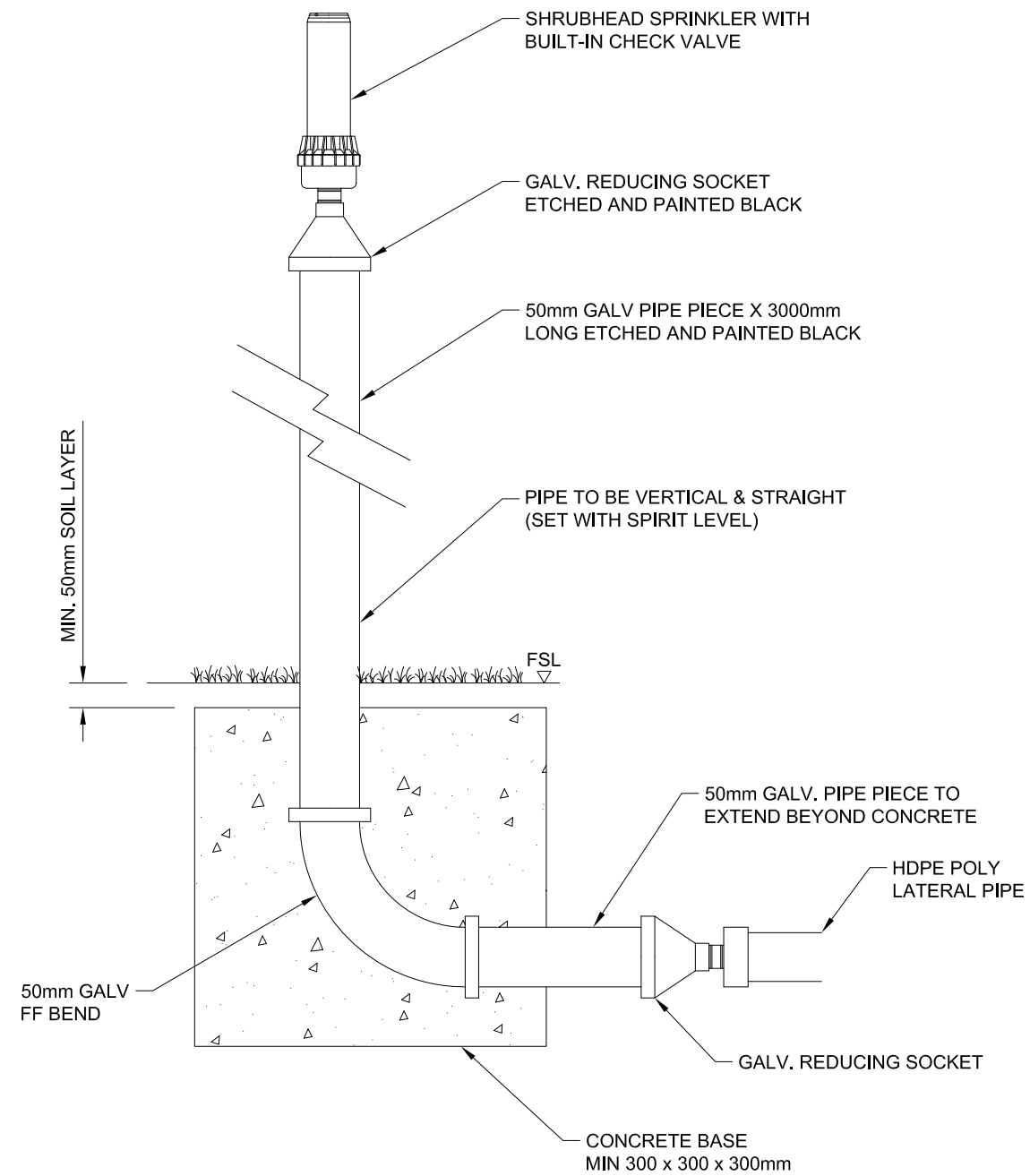
TYPICAL RIGID RISER INSTALLATION
