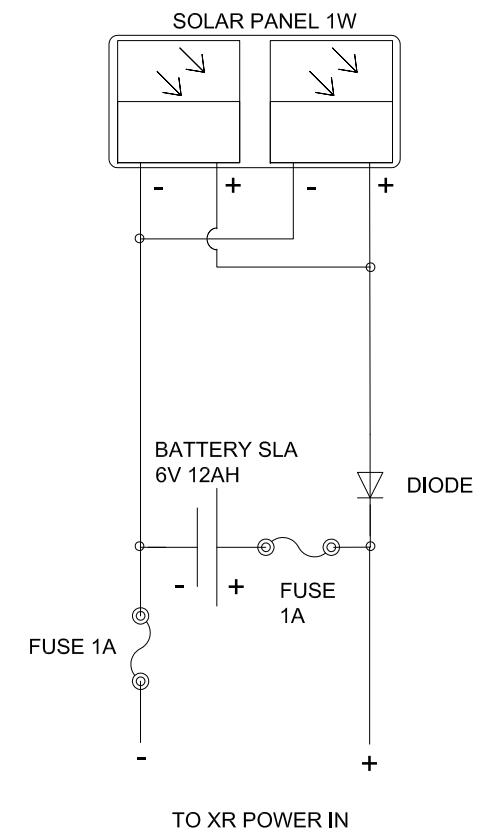
INPUT POWER WIRING DIAGRAM
