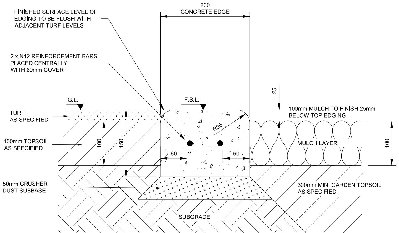
CONCRETE GARDEN EDGING SCALE 1:5
