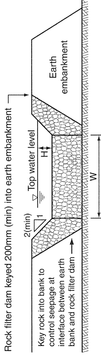
(e) Rock filter dam with overflow spill
