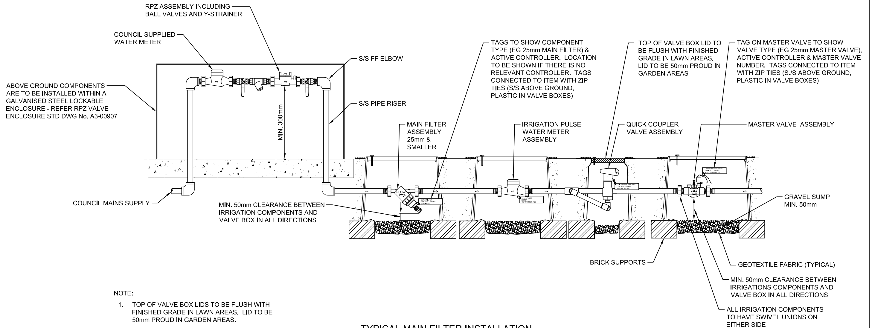
TYPICAL MAIN FILTER INSTALLATION UNDERGROUND (25mm AND SMALLER)
