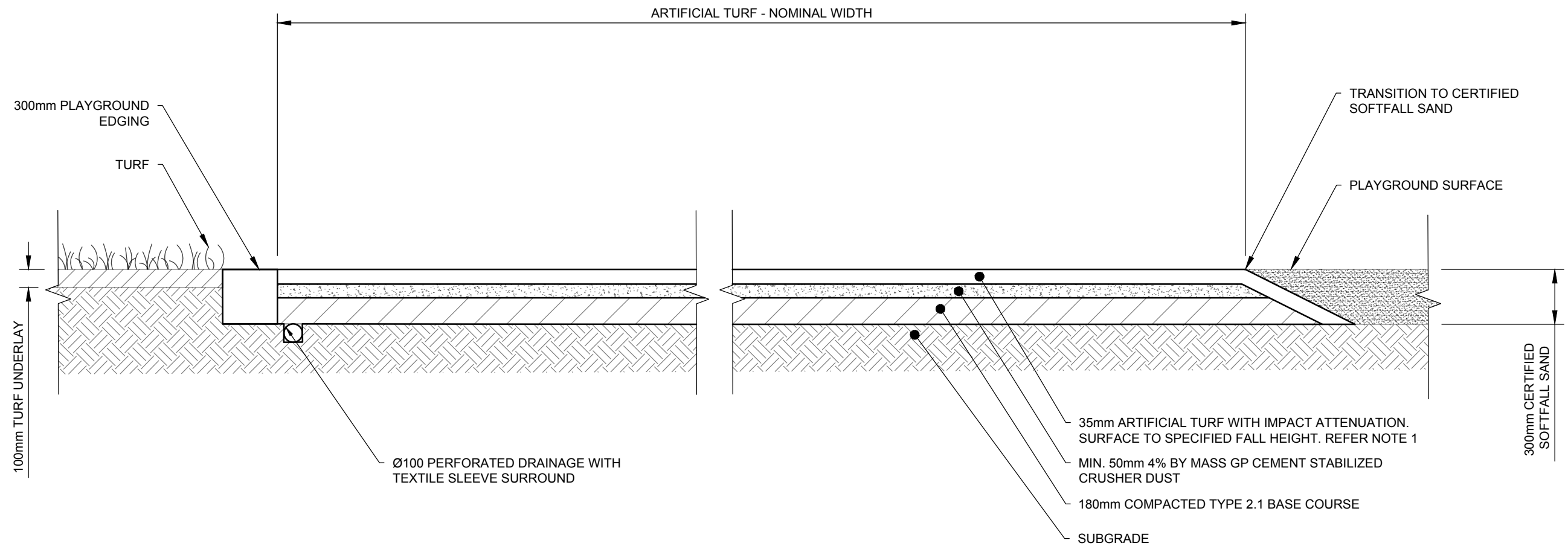
PLAYGROUND SOFTFALL TREATMENT - ARTIFICIAL TURF SCALE 1:25
