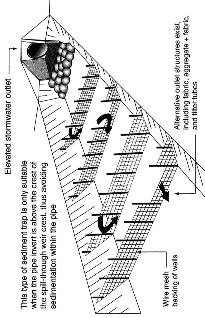
(a) Coarse sediment trap outlet system
