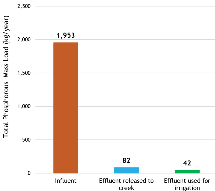
Figure 5-7 SWRF Influent and Effluent Phosphorous Mass Loads for 2022-2023 FY
