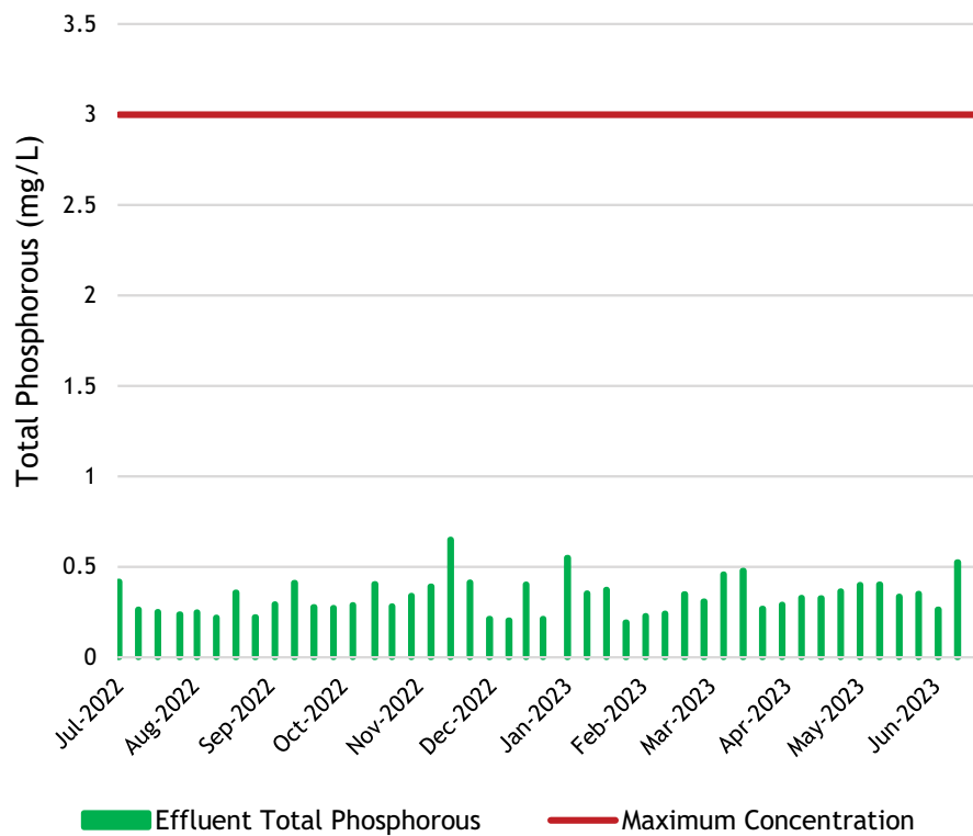
Figure 5-4 SWRF Effluent Phosphorous Concentrations for 2022-2023 FY
