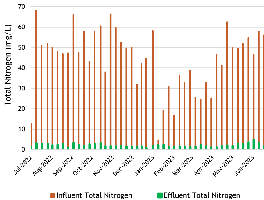
Figure 5-1 SWRF Influent and Effluent Nitrogen Concentrations for 2022-2023 FY
