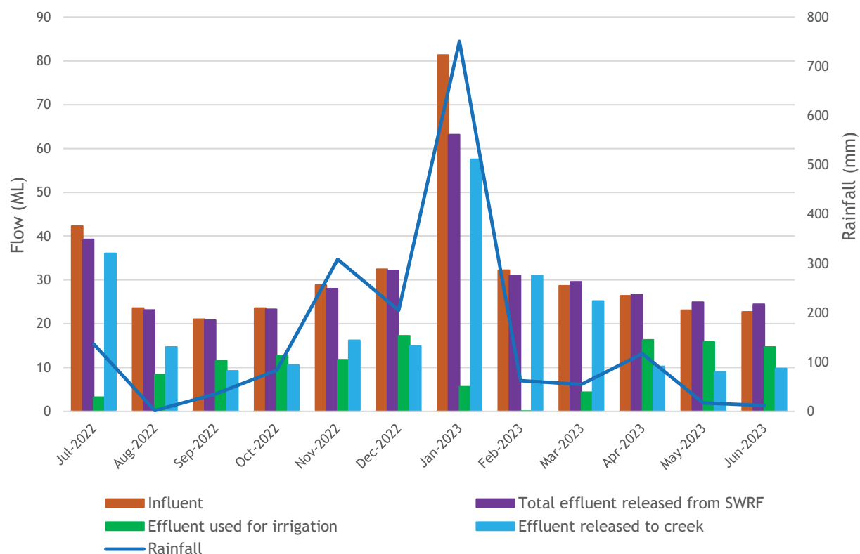
Figure 4-1 SWRF Monthly Influent and Effluents Flows and Rainfall for 2022-2023 FY
