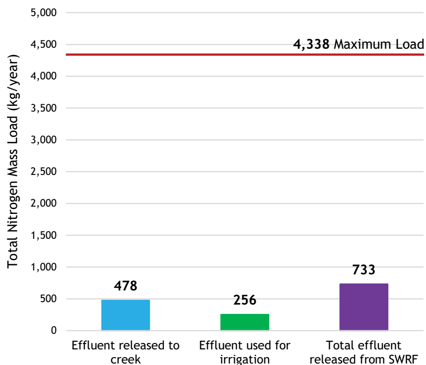
Figure 5-6 SWRF Effluent Nitrogen Mass Loads for 2022-2023 FY
