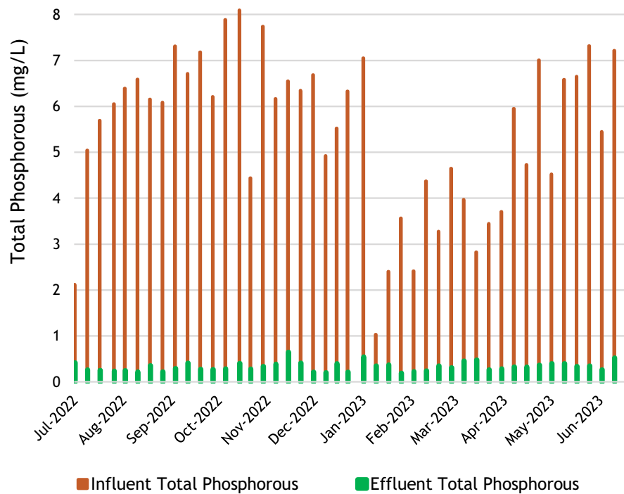
Figure 5-3 SWRF Influent and Effluent Phosphorous Concentrations for 2022-2023 FY
