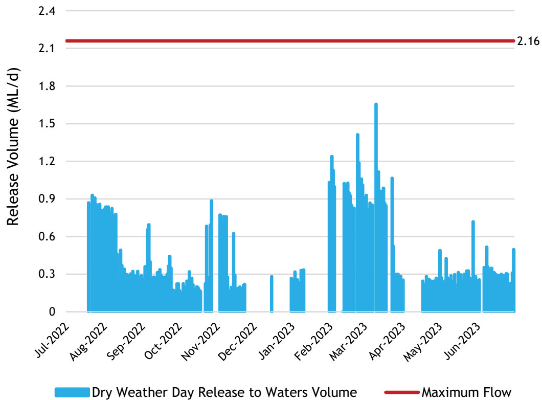
Figure 4-2 SWRF Dry weather day release to waters volume for 2022-2023 FY
