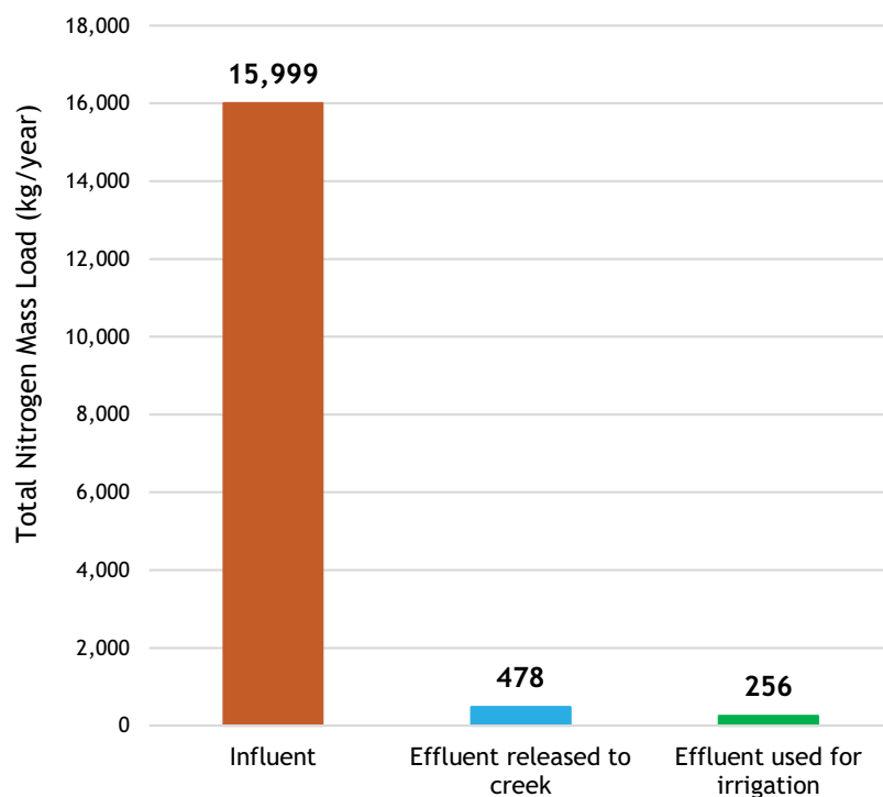
Figure 5-5 SWRF Influent and Effluent Nitrogen Mass Loads for 2022-2023 FY
