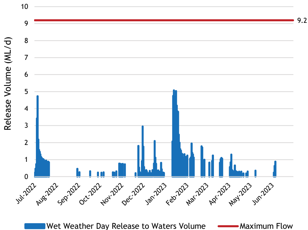
Figure 4-3 SWRF Wet weather day release to waters volume for 2022-2023 FY
