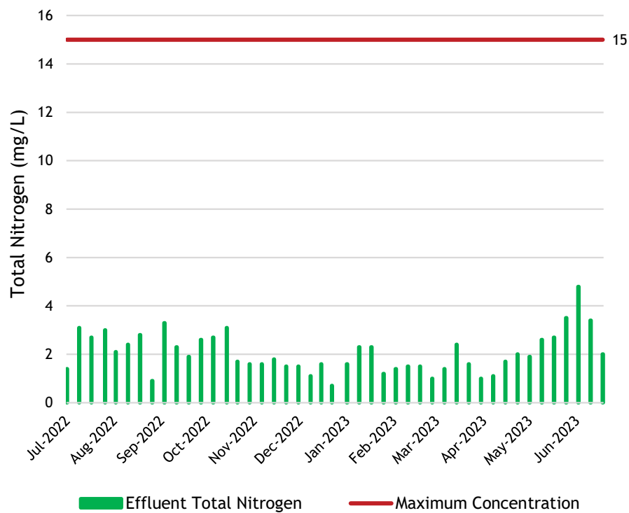
Figure 5-2 SWRF Effluent Nitrogen Concentrations for 2022-2023 FY
