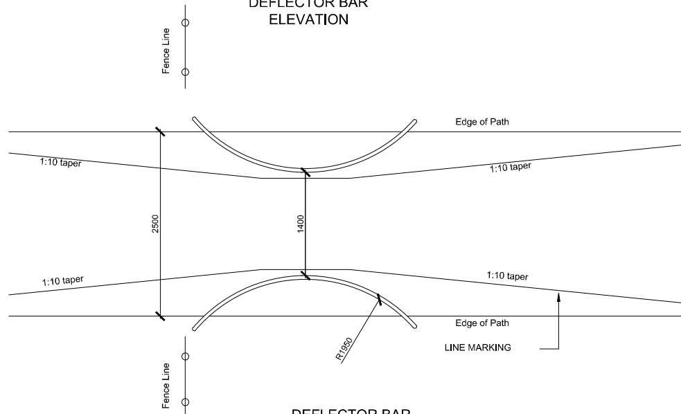
DEFLECTOR BAR PLAN
