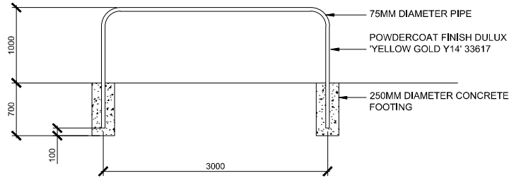
DEFLECTOR BAR ELEVATION
