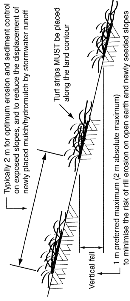
(c) Placement of grass filter strips along the contour of a slope
