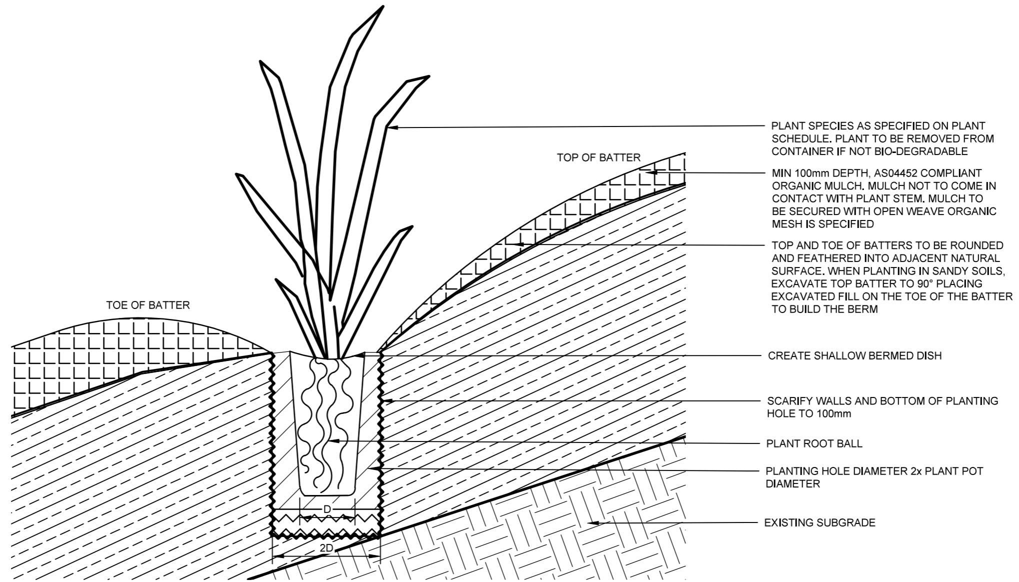
TYPICAL DETAIL - TUBE STOCK BATTER PLANTING NTS
