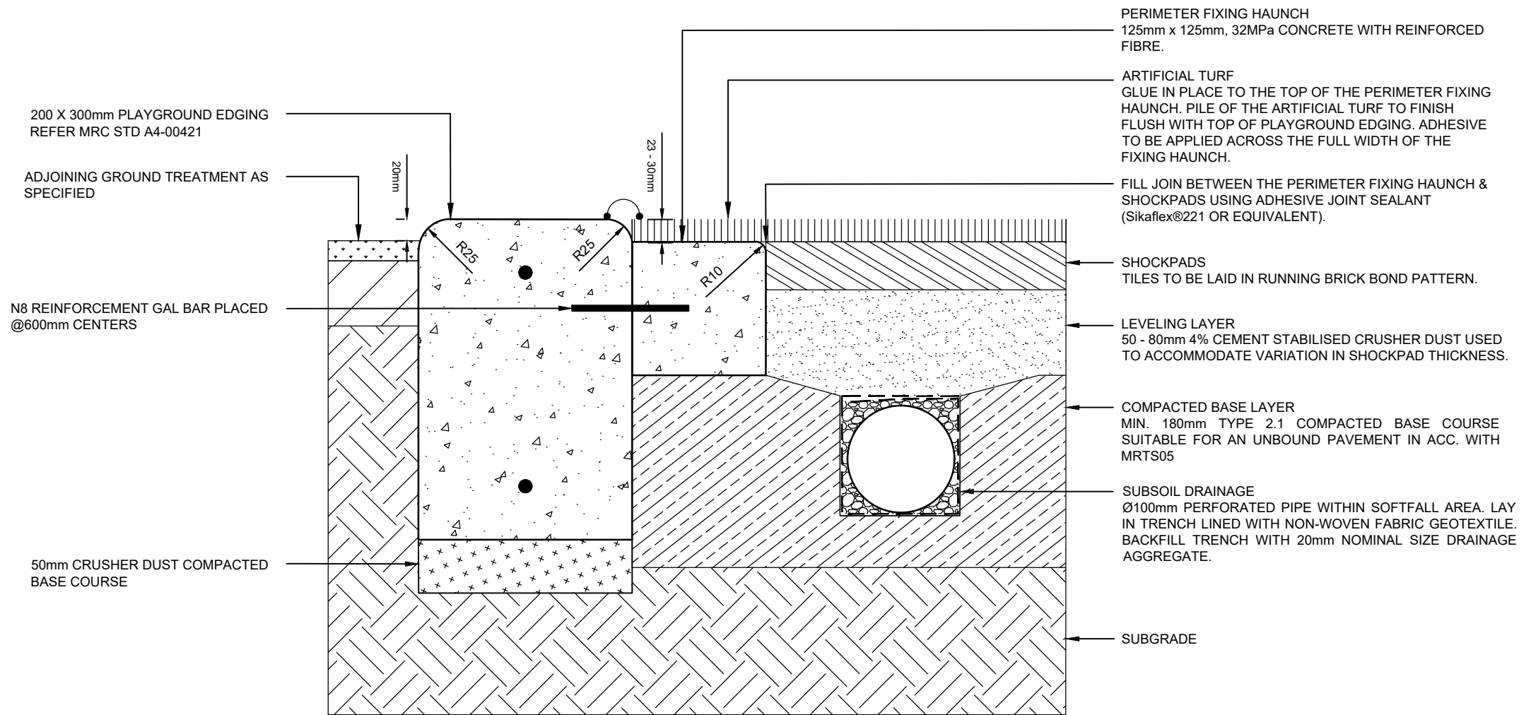
PLAYGROUND EDGING WITH ARTIFICIAL TURF SOFTFALL
